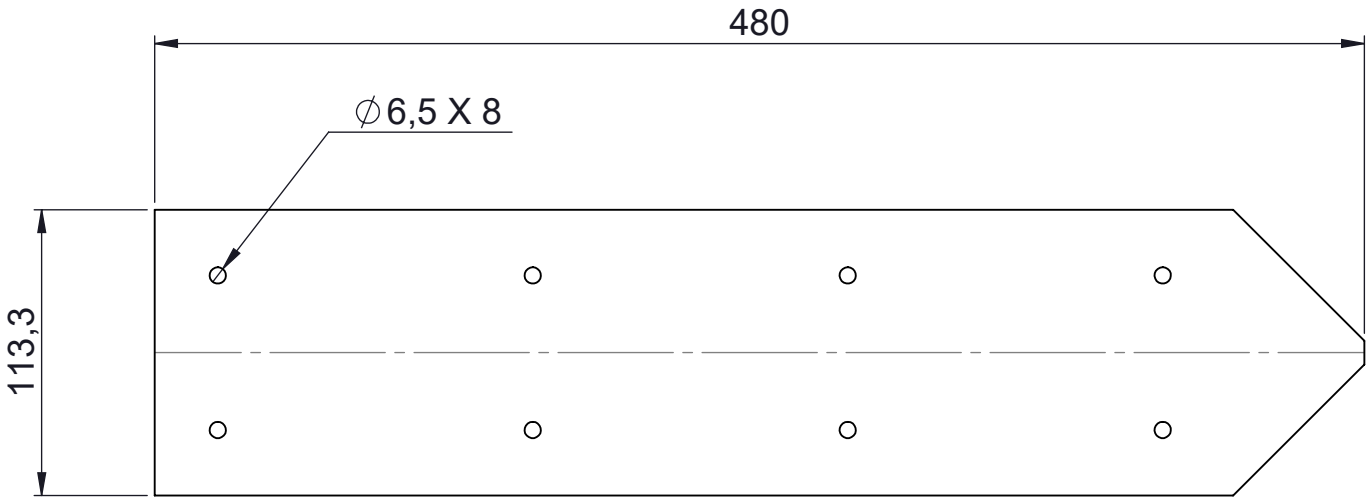
FLAT PATTERN
