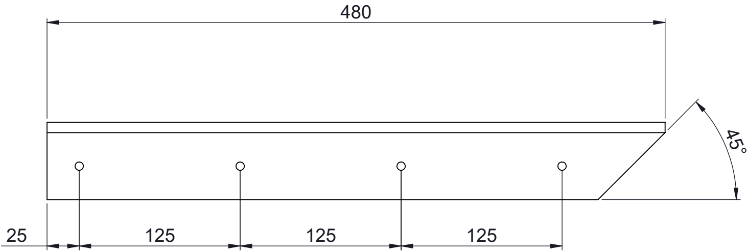
FRONT VIEW
