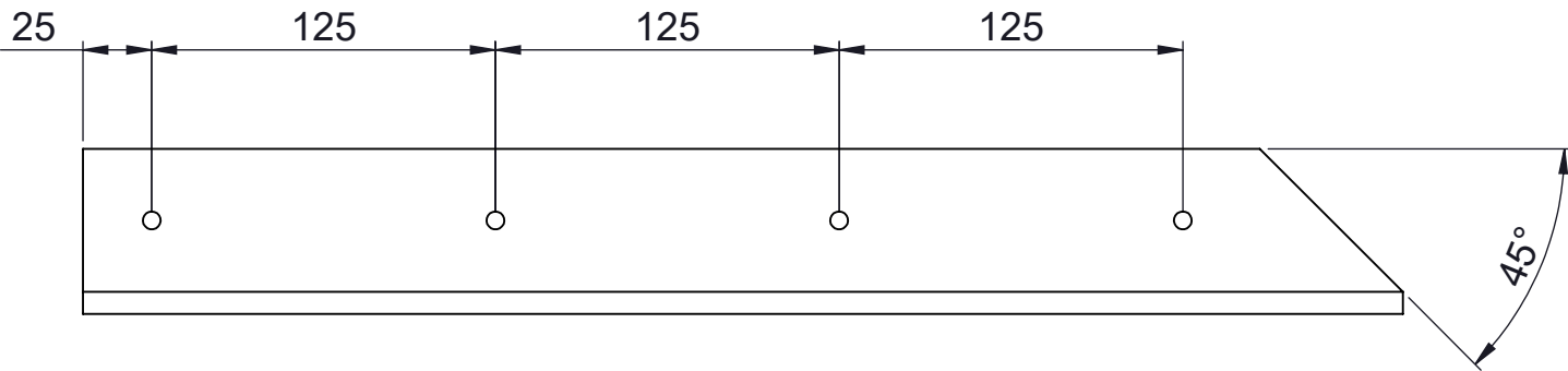
TOP VIEW
